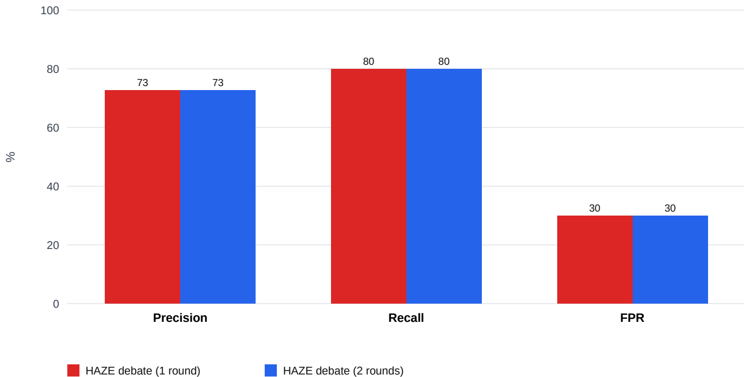
Figure 2. Precision / Recall / FPR by condition
